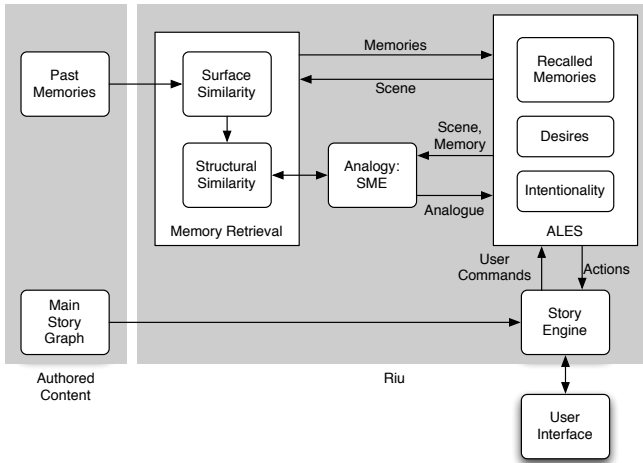
Fig. 3. Riu's system architecture.
