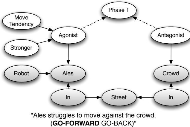
Fig. 4. A force-dynamics-based representation of a scene in the Riu system.
